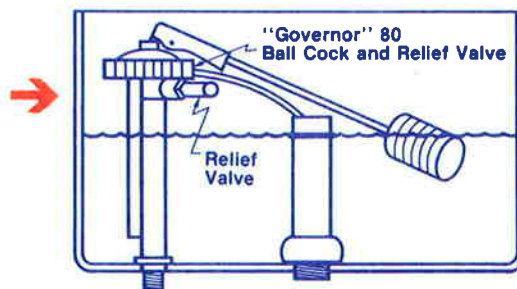
TYPICAL WATER CLOSET
